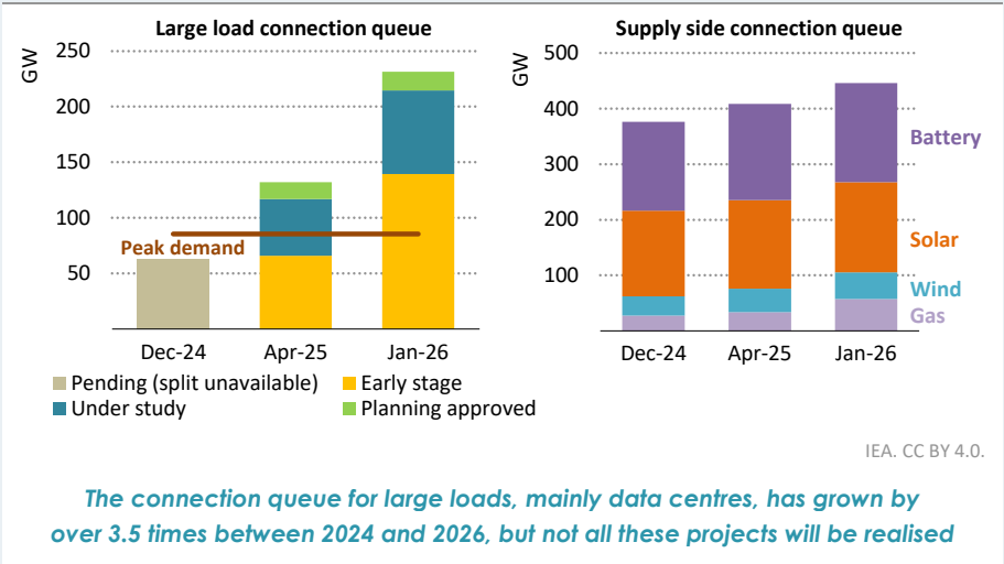
Figure 1.6 ▶ Connection queue in ERCOT
