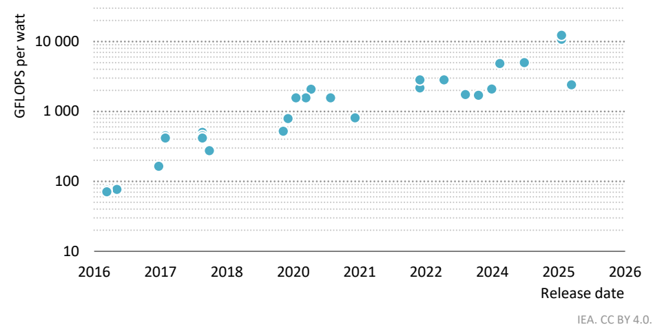
Figure 2.2 ▶ Energy efficiency of leading machine learning hardware, 2016-2025
