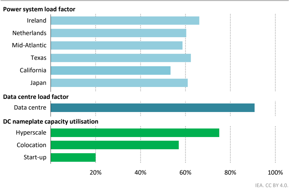
Figure 8.5 ▶ Load and capacity utilisation factors of data centres and at power system level
