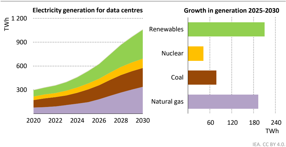
Figure 5.4 ▶ Global electricity generation for data centres, 2020-2030
