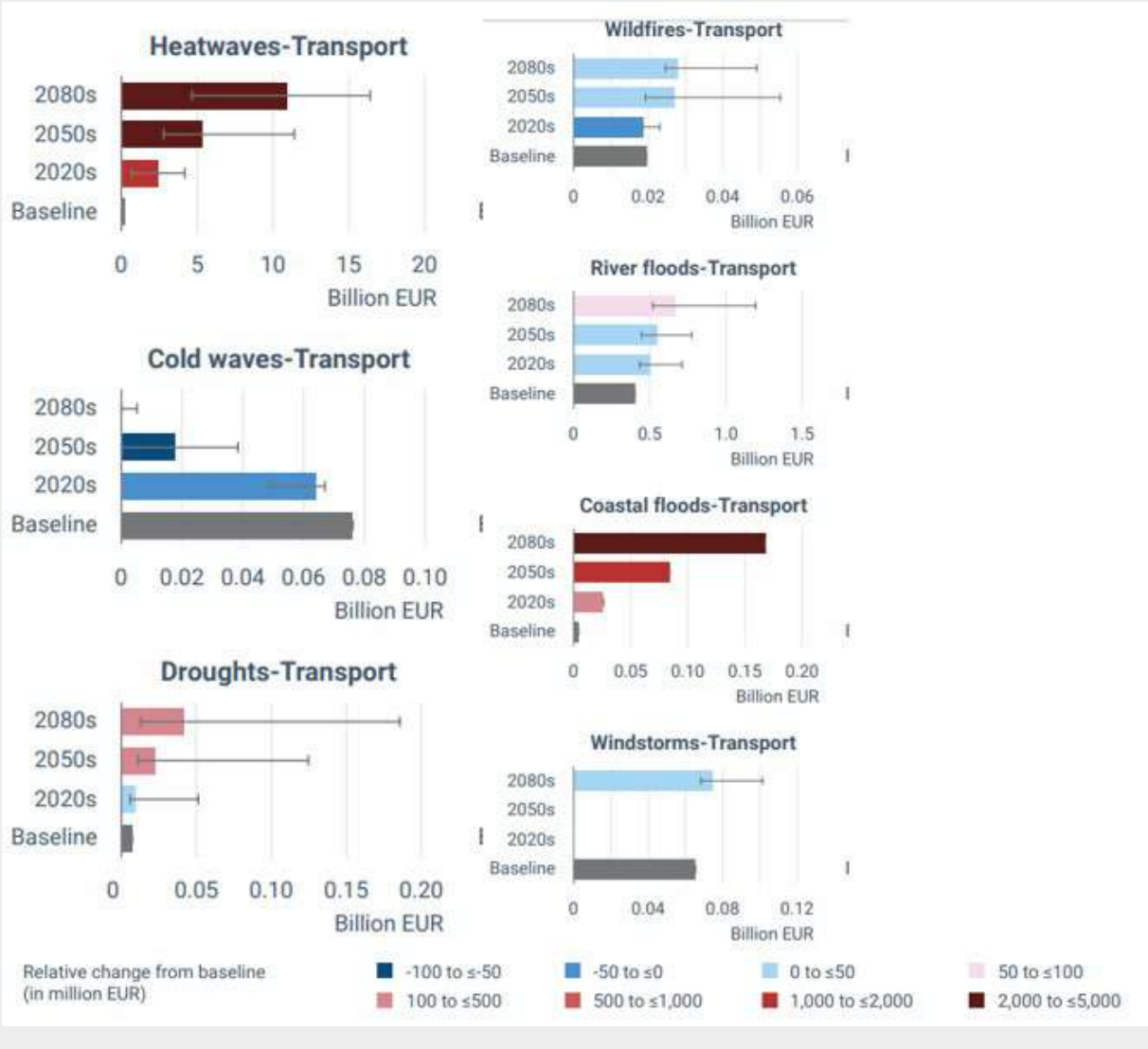
Figure 20: Expected annual damage to critical infrastructure assets, European Climate Risk Assessment, European Environment Agency, 2024
