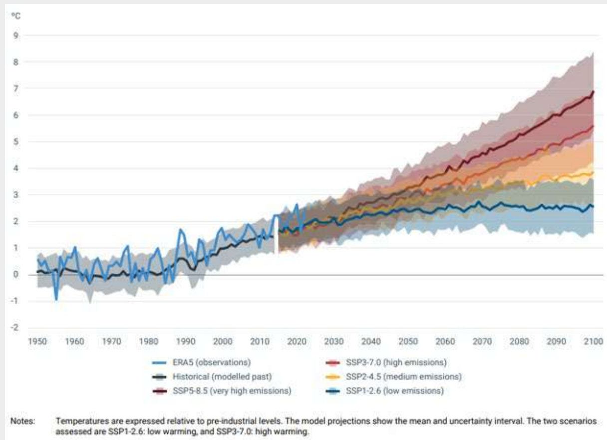
Figure 22: Observed and projected temperature increase over European land area, European Climate Risk Assessment, European Environment Agency, 2024
