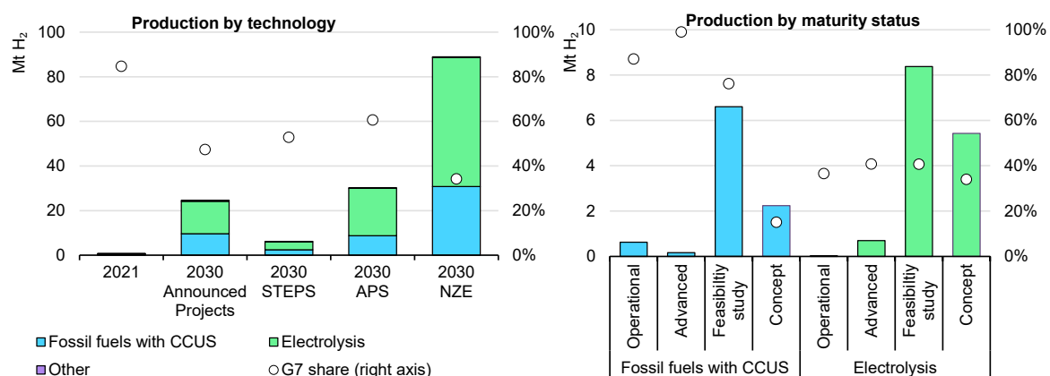
Figure 1.10 Global low-emission hydrogen production and G7 share based on announced projects and by scenario, 2021 and 2030
