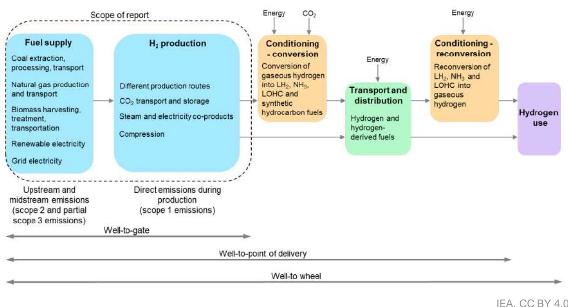
Figure 2.1 Scope and system boundaries for emissions accounting schemes
