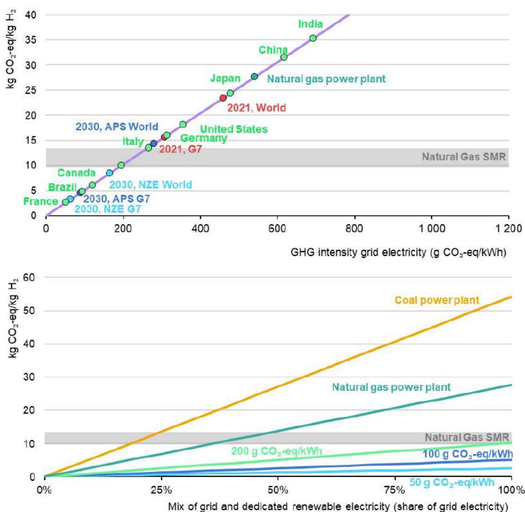
Figure 2.4 Impact of the emissions intensity of grid electricity and of the mix of grid and dedicated renewable electricity on the emissions intensity of hydrogen
