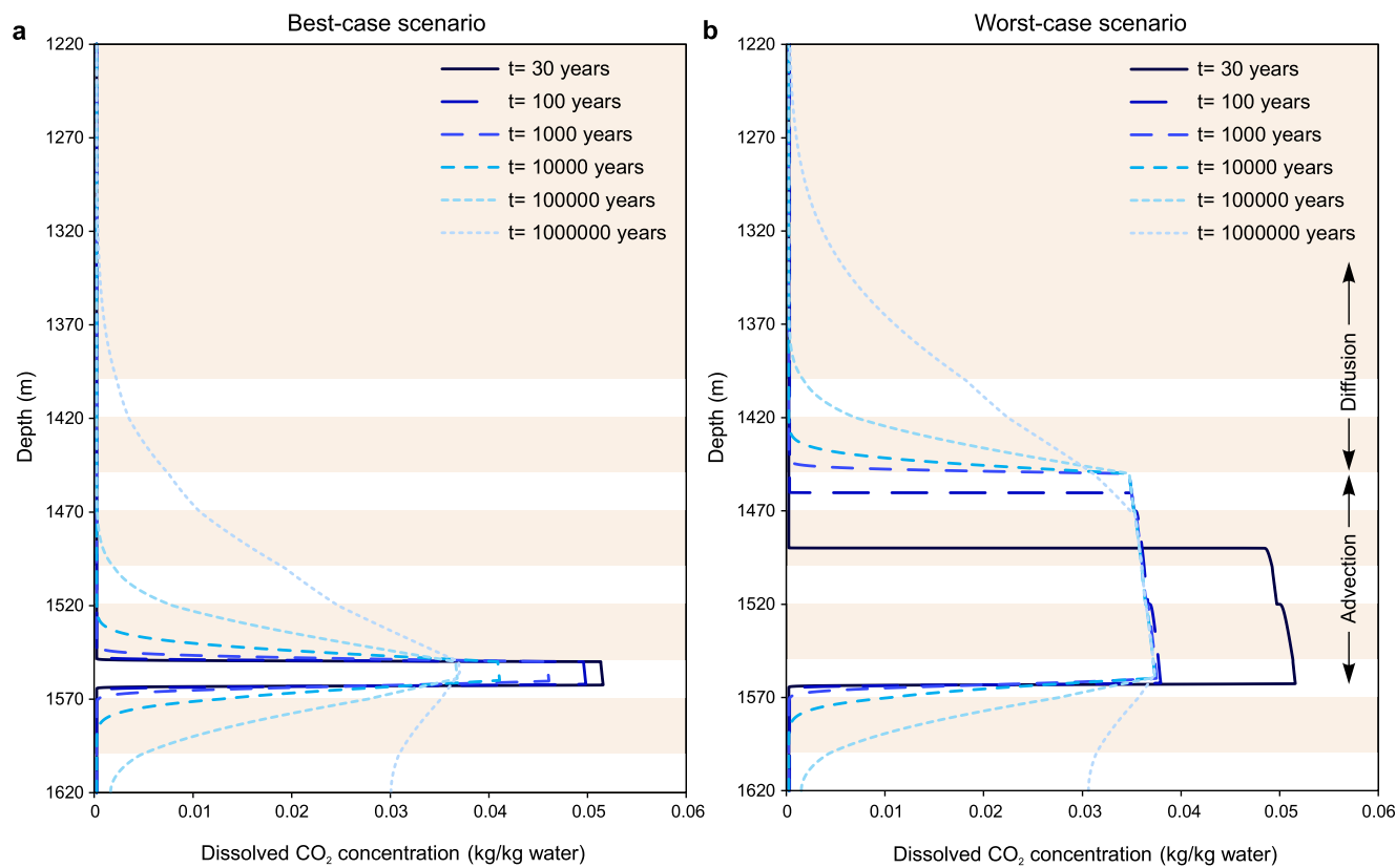
Figure 3. Dissolved CO 2 concentration profiles. Temporal evolution of the CO 2 concentration along a sequence of aquifers and caprocks for the (a) best-case and (b) worst-case leakage assessment scenarios.
