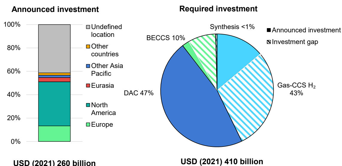
Figure 4.13 Announced global cumulative investment in large-scale, site-tailored clean energy technologies by region/country and that required to meet demand in 2030 in the NZE Scenario, 2022-2030
