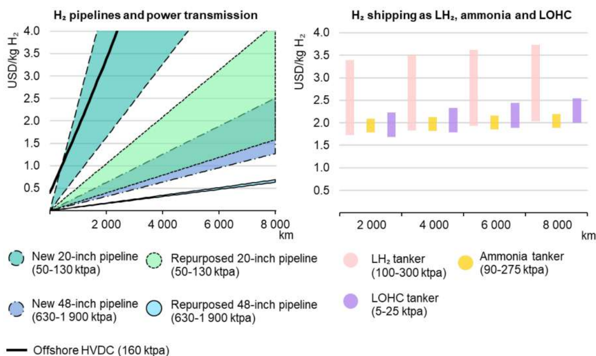
Figure 5.22 Indicative levelised cost of delivering hydrogen, by transport option and distance in the NZE Scenario, 2030
