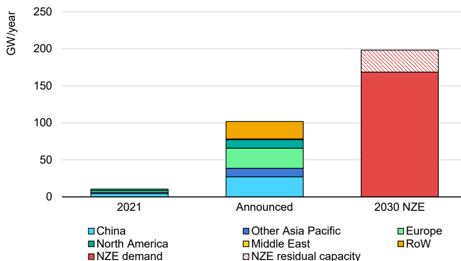
Figure 4.12 Electrolyser manufacturing capacity by country/region according to announced projects and in the NZE Scenario
