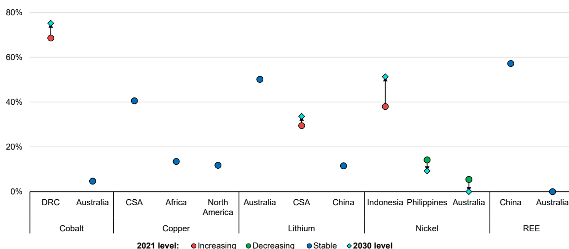
Figure 3.9 Shares of the leading regions in global mining of selected critical minerals in 2021 and 2030 based on currently anticipated investments
