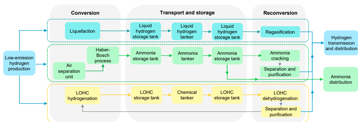
Figure 5.13 Technological pathways for long-distance transport for the supply of hydrogen and ammonia by tanker
