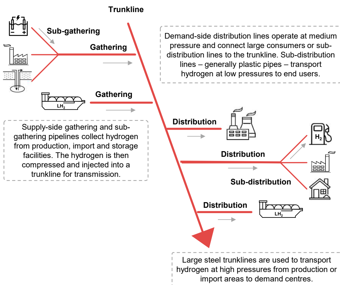
Figure 5.12 Hydrogen pipeline network configuration
