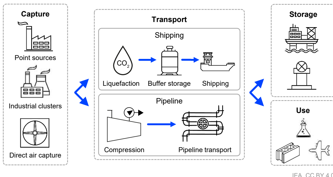
Figure 5.29 CO 2 flows through the CO 2 management value chain
