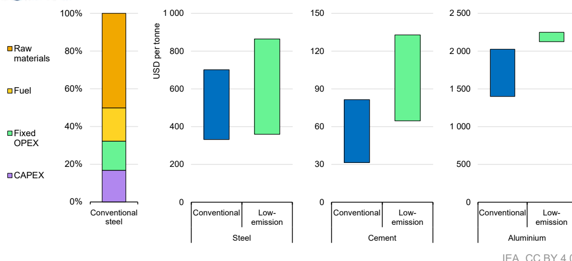
Figure 1.13 Indicative levelised cost of production for selected bulk materials
