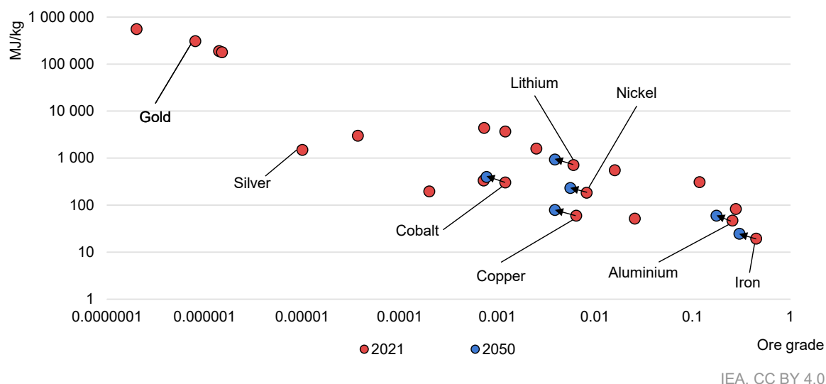
Figure 3.10 Global energy intensity and average grade of ore production for selected metals
