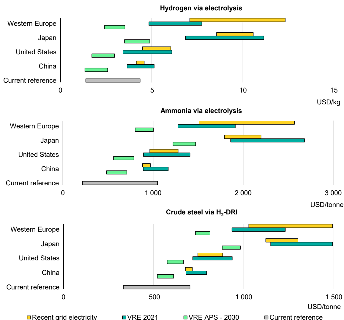
Figure 6.12 Indicative production costs for hydrogen and hydrogen-based commodities produced via electrolysis
