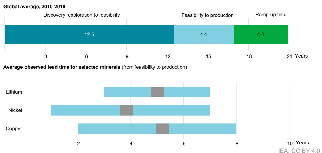
Figure 1.15 Lead times for mining of selected minerals
