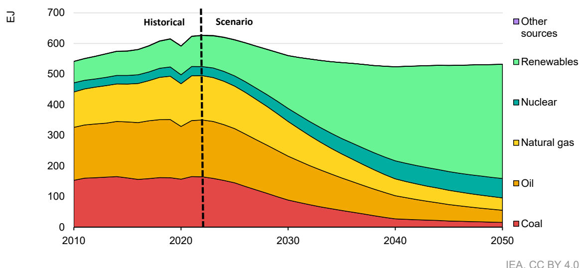
Figure 1.2 Global total primary energy supply in the NZE Scenario
