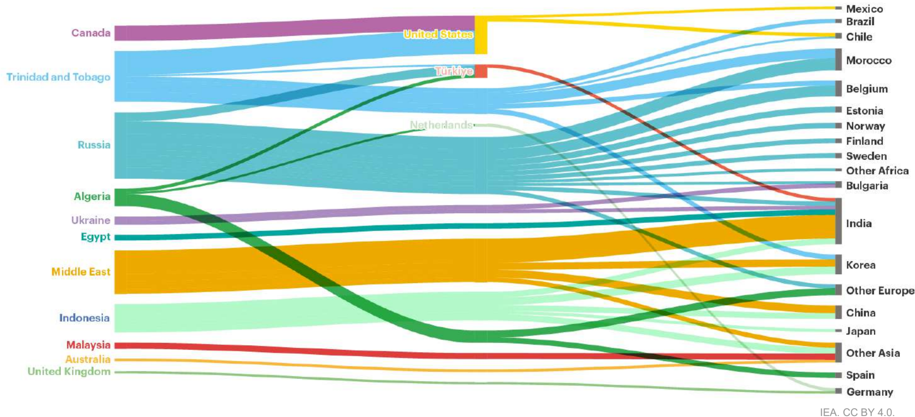
Figure 5.21 International ammonia trade flows via shipping, 2019
