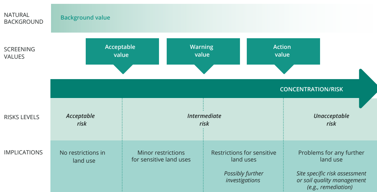
Figure 5.2 Schematic representation of thresholds (adopted from the Heracles network)
