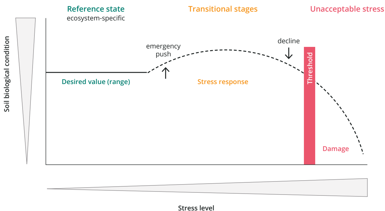
Figure 6.1 Baseline and threshold approach for soil biodiversity monitoring
