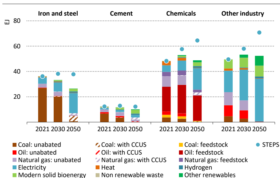
Figure 3.12 ► Final energy consumption by source in industry sub-sectors in the NZE Scenario, 2021-2050
