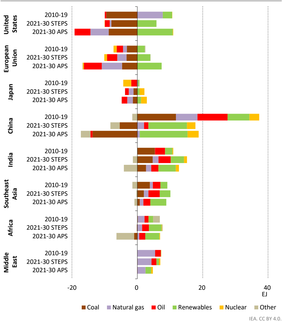
Figure 5.3 ▶ Change in total energy supply by region, fuel and scenario, 2010-2019 and 2021-2030
