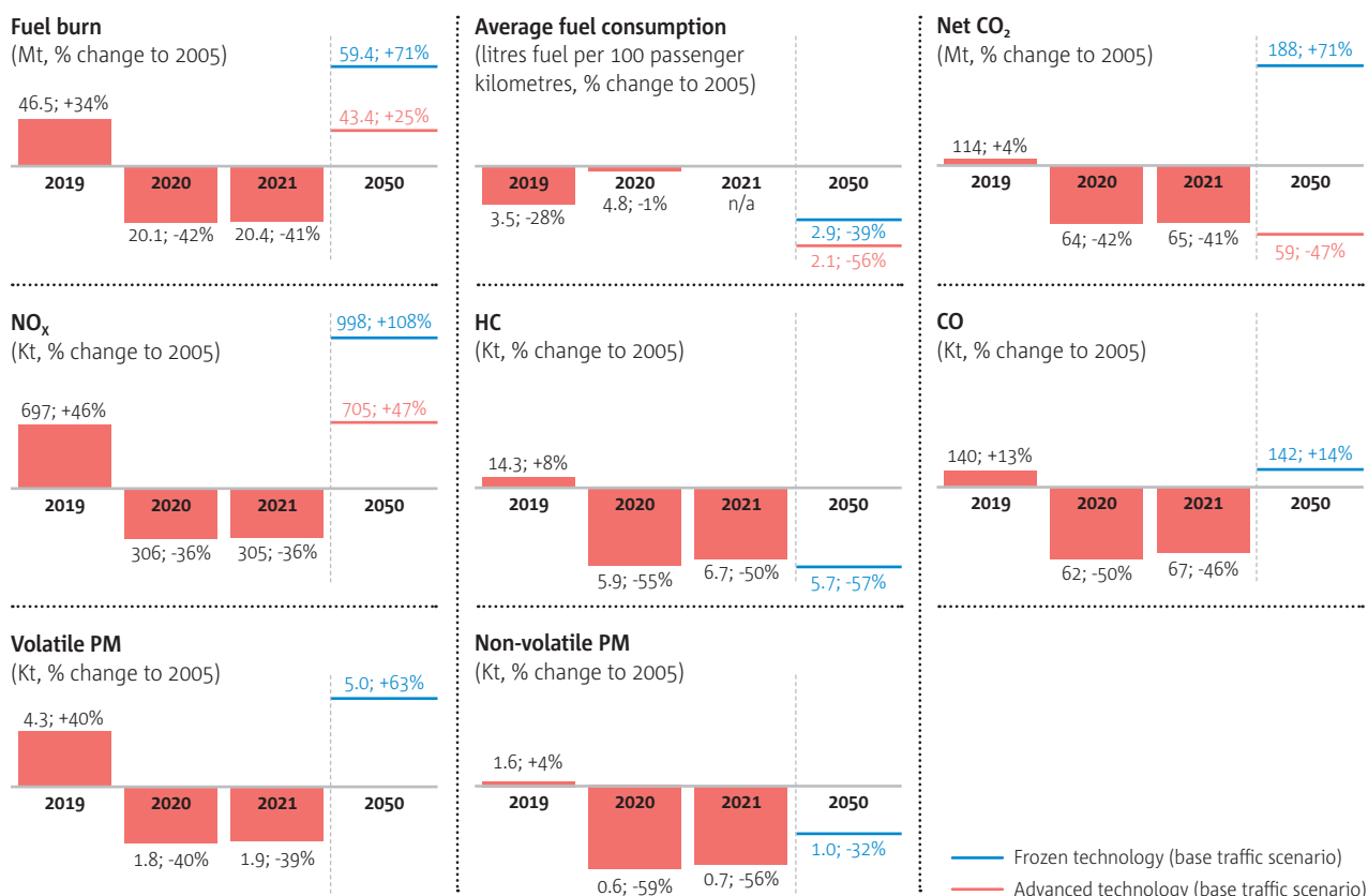
Figure 1.15 Summary of full-flight emission indicators (% change to 2005)
