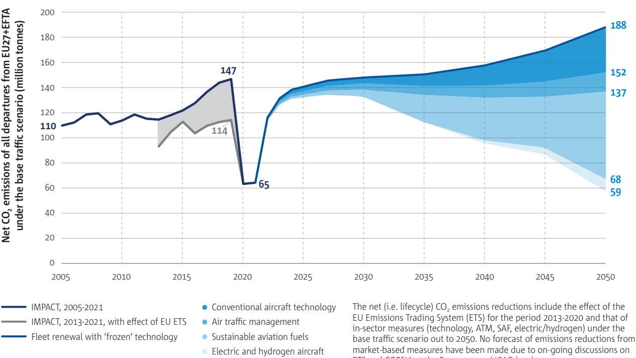
Figure 1.10b Net CO 2 emissions could be halved by 2050 using sustainable aviation fuels
