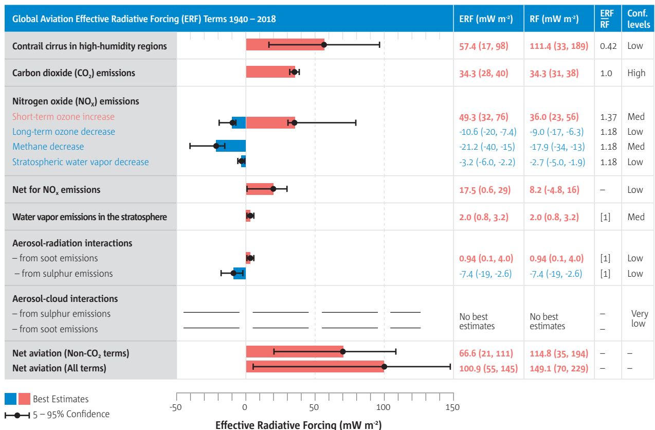
Figure 2.5 Best-estimates for climate forcing terms from global aviation from 1940 to 2018 [32]
