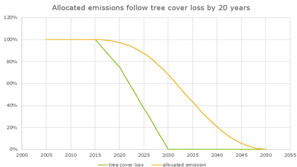
Figure 5. Deforestation and deforestation emissions pathways
