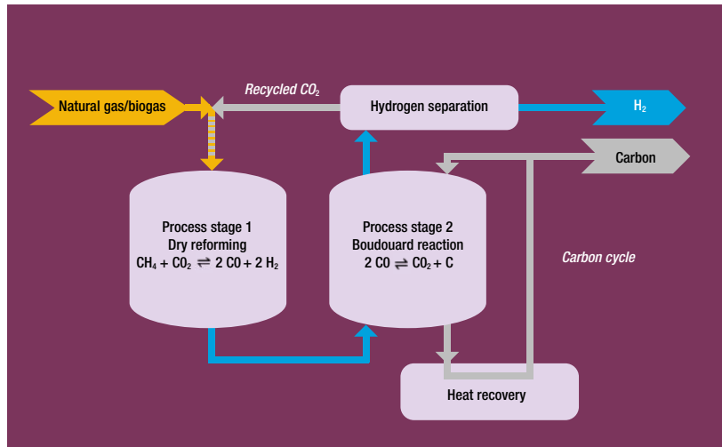
Schematic diagram of the two-stage process under investigation
