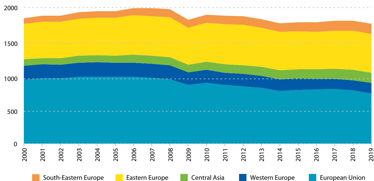
Figure 9 Territorial fossil CO 2 emissions by subregion, 2000–2019 (Millions of tons of CO 2 )
