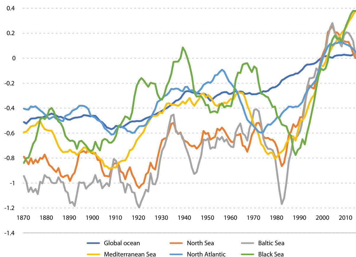
Figure 24 Time series of annual average sea surface temperature, referenced to average temperature between 1993 and 2012 (°C)
