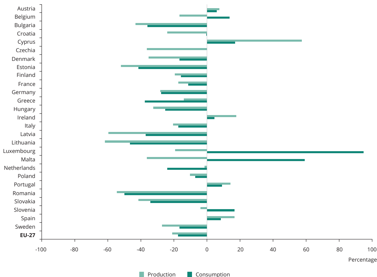
Figure 2.4 Percentage change in national GHG emissions (1990-2018) in the EU-27, from production and consumption perspectives
