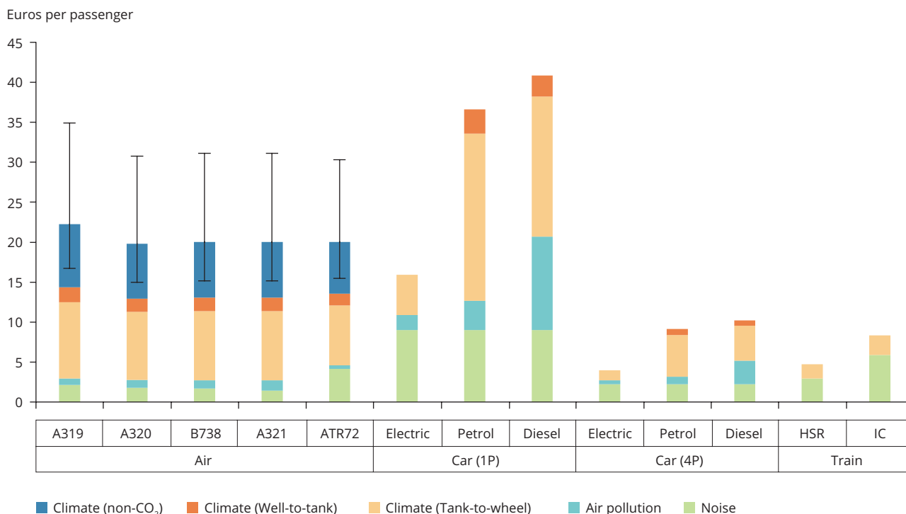
Figure 5.3 Emission costs of different transport modes (1 000 km)
