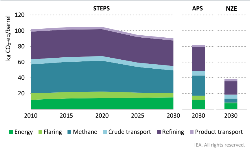
Figure 5.9 ▶ Global average emissions intensity of oil production
