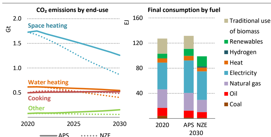
Figure 3.24 ▶ CO 2 emissions by end-use and final energy consumption by fuel in the buildings sector in the Announced Pledges and Net Zero Emissions by 2050 scenarios
