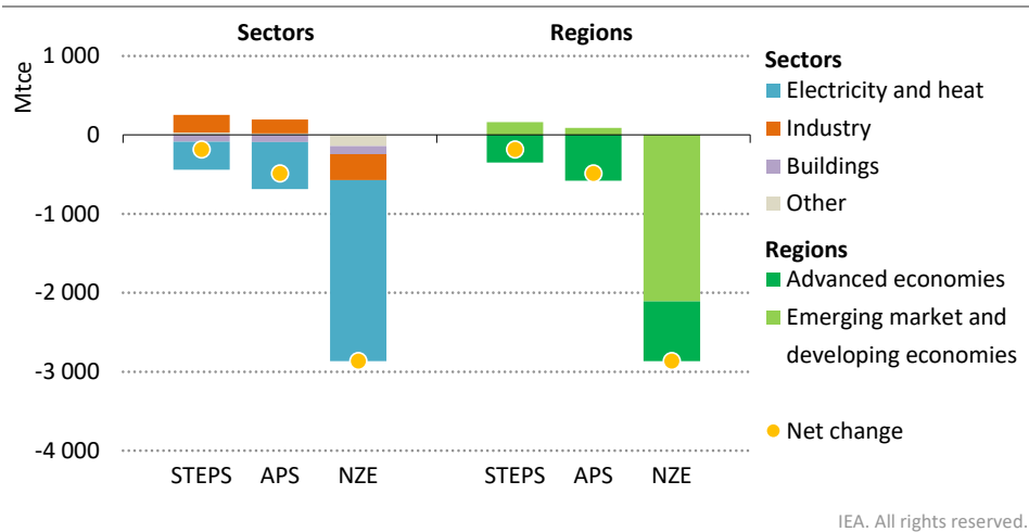
Figure 5.25 ► Change in coal demand by scenario between 2020 and 2030
