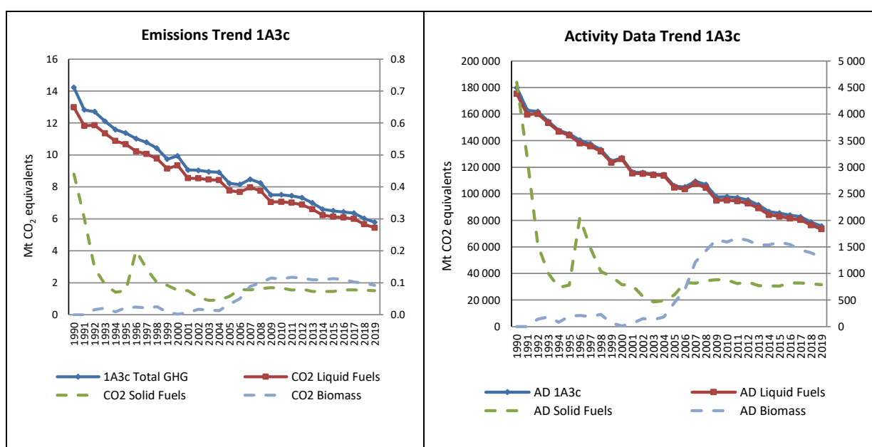
Figure 3.131 1A3c Railways: CO 2 Emission Trend and Activity Data
