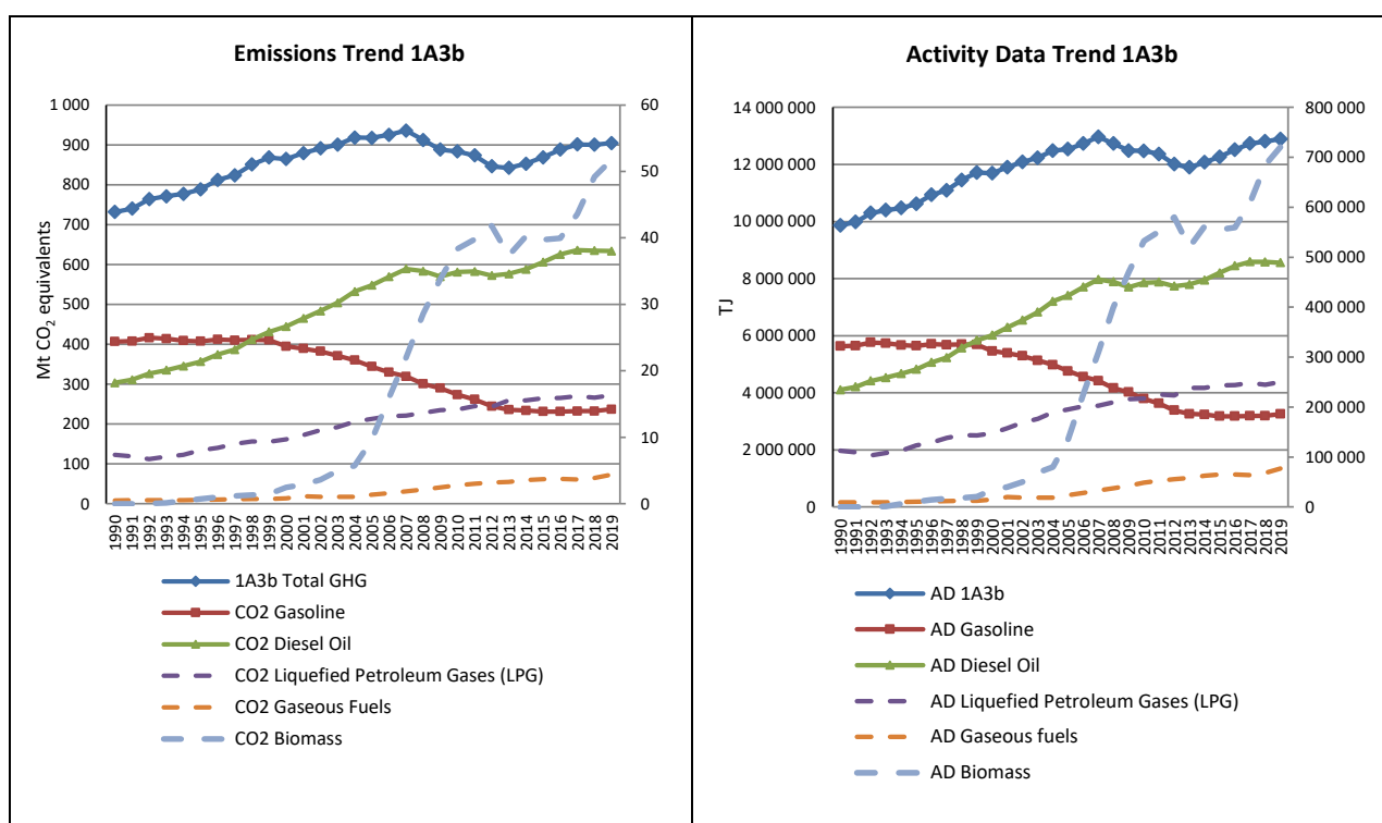
Figure 3.111 1A3b Road Transport: CO 2 Emission Trend and Activity Data
