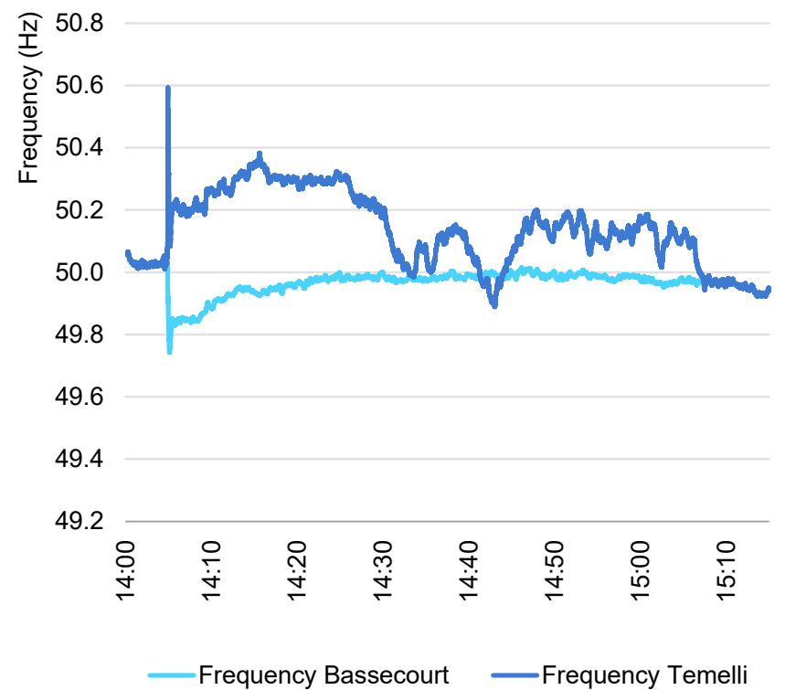
Frequency during the event
