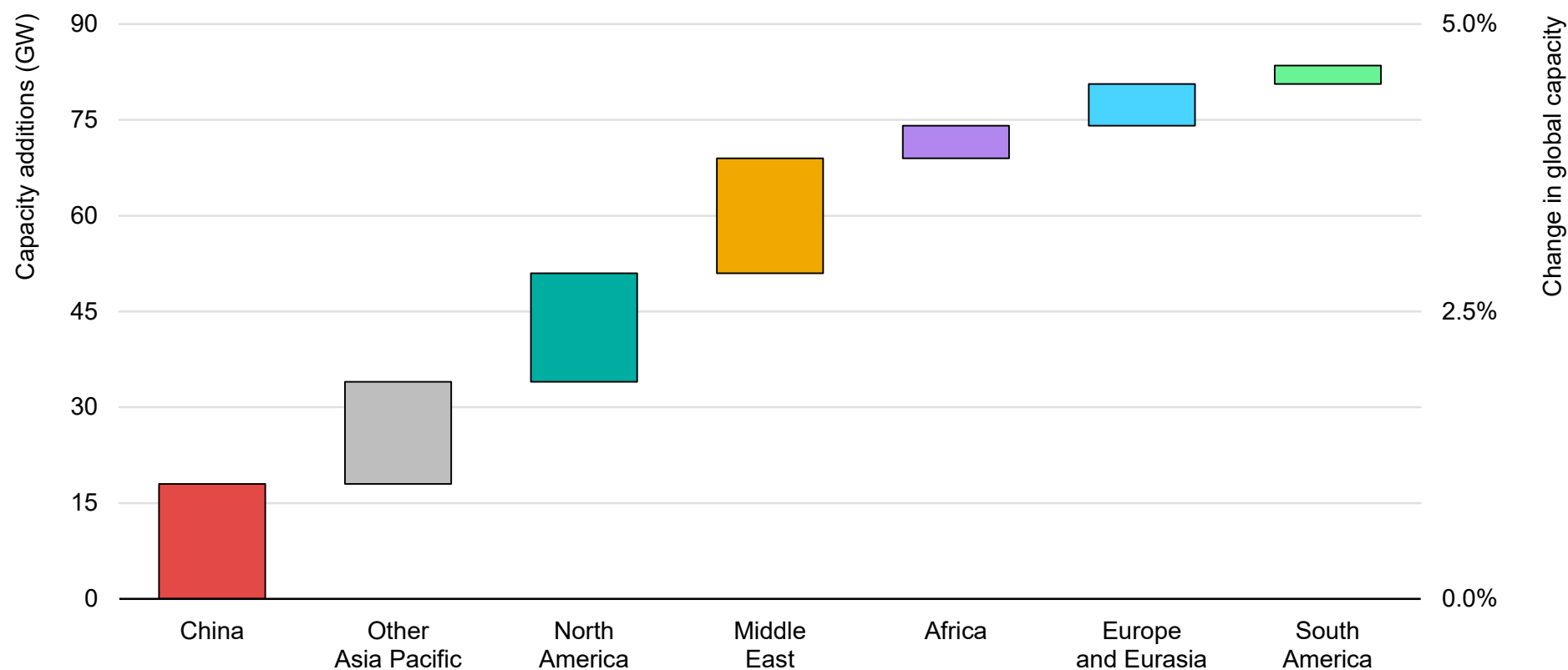
Gas-fired power generation capacity additions by region, 2020-2022
