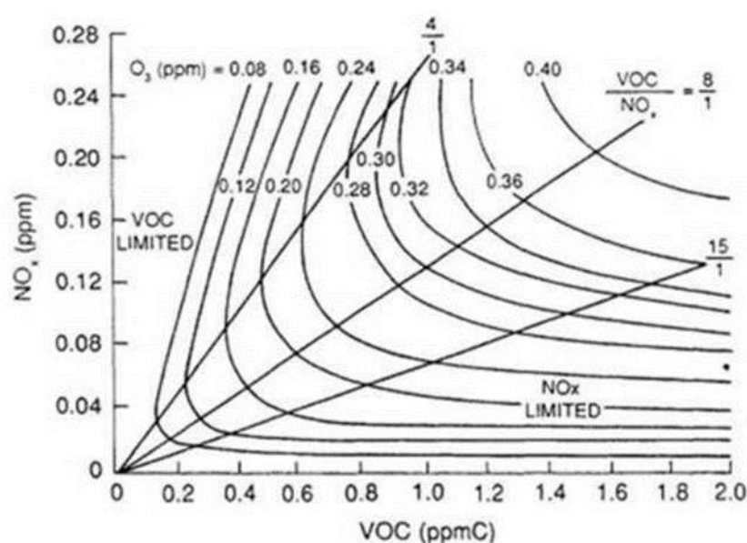
Figure 11: The theoretical formation of O 3 as a function of NO x and NMVOCs and of the ratio VOC/NO x (Source: NRC book "Rethinking the Ozone problem in urban and regional air pollution")
