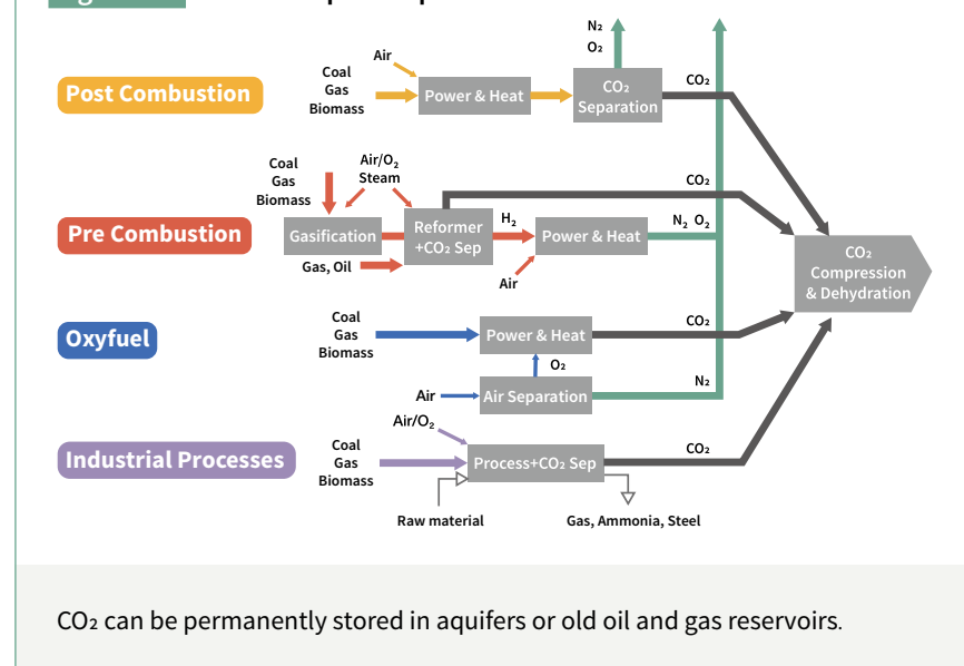
Figure 2.1 Carbon capture options
