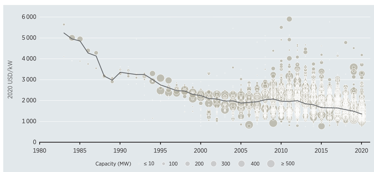
Figure 2.4 Total installed costs of onshore wind projects and global weighted-average, 1983-2020
