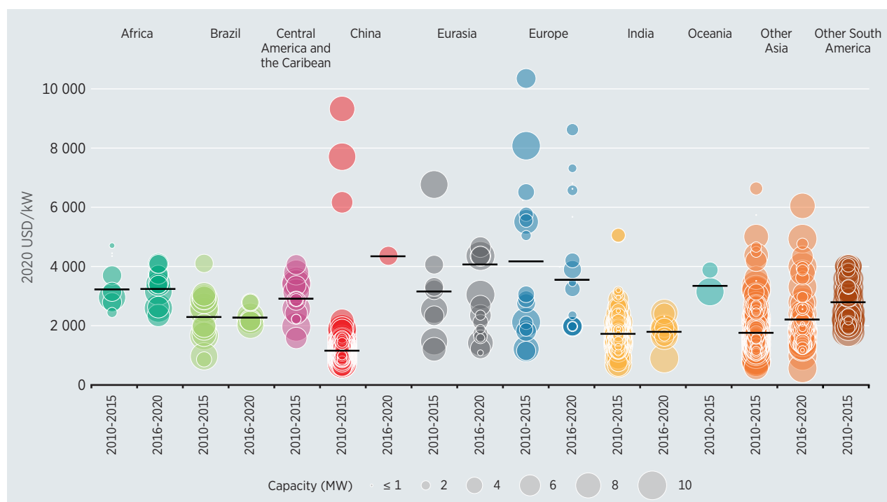
Figure 6.6 Total installed costs by project and capacity weighted averages for small hydropower projects by country/region, 2010-2020
