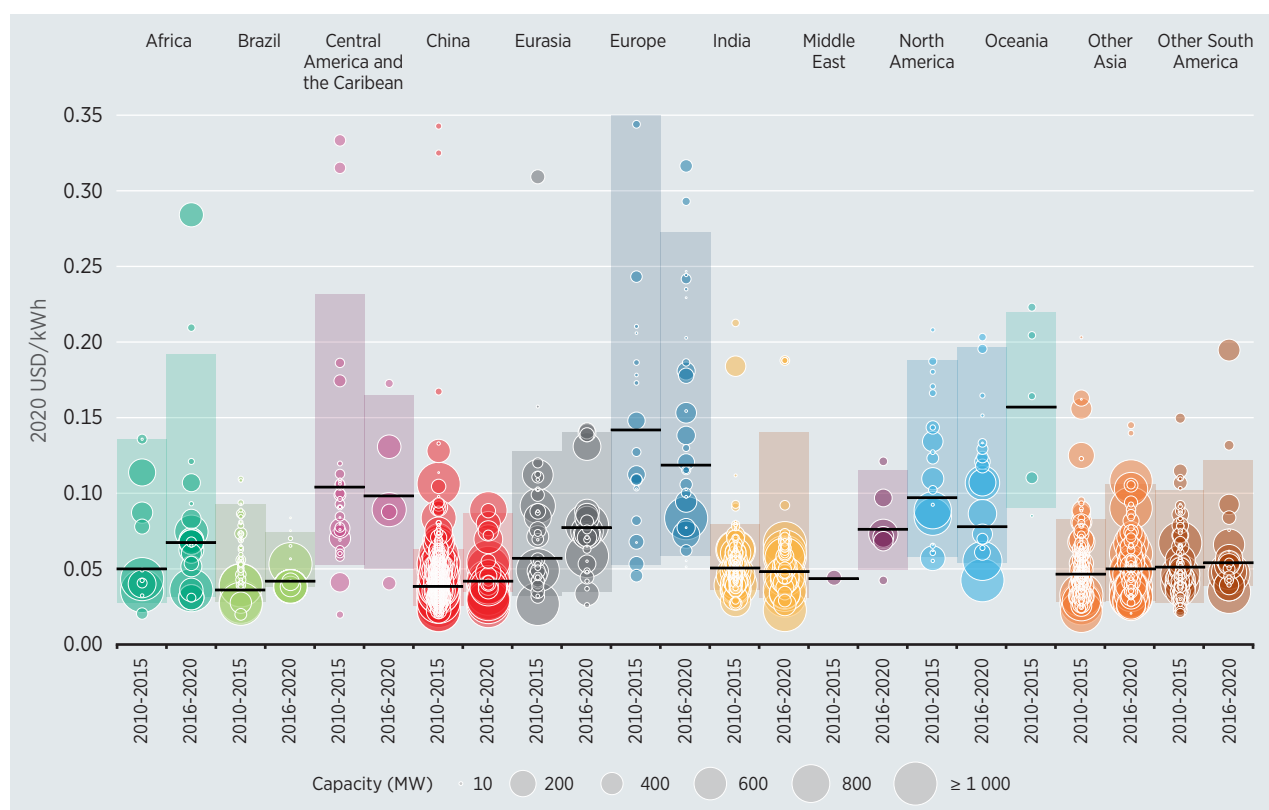
Figure 6.7 Large hydropower project LCOE and capacity weighted averages by country/region, 2010-2020
