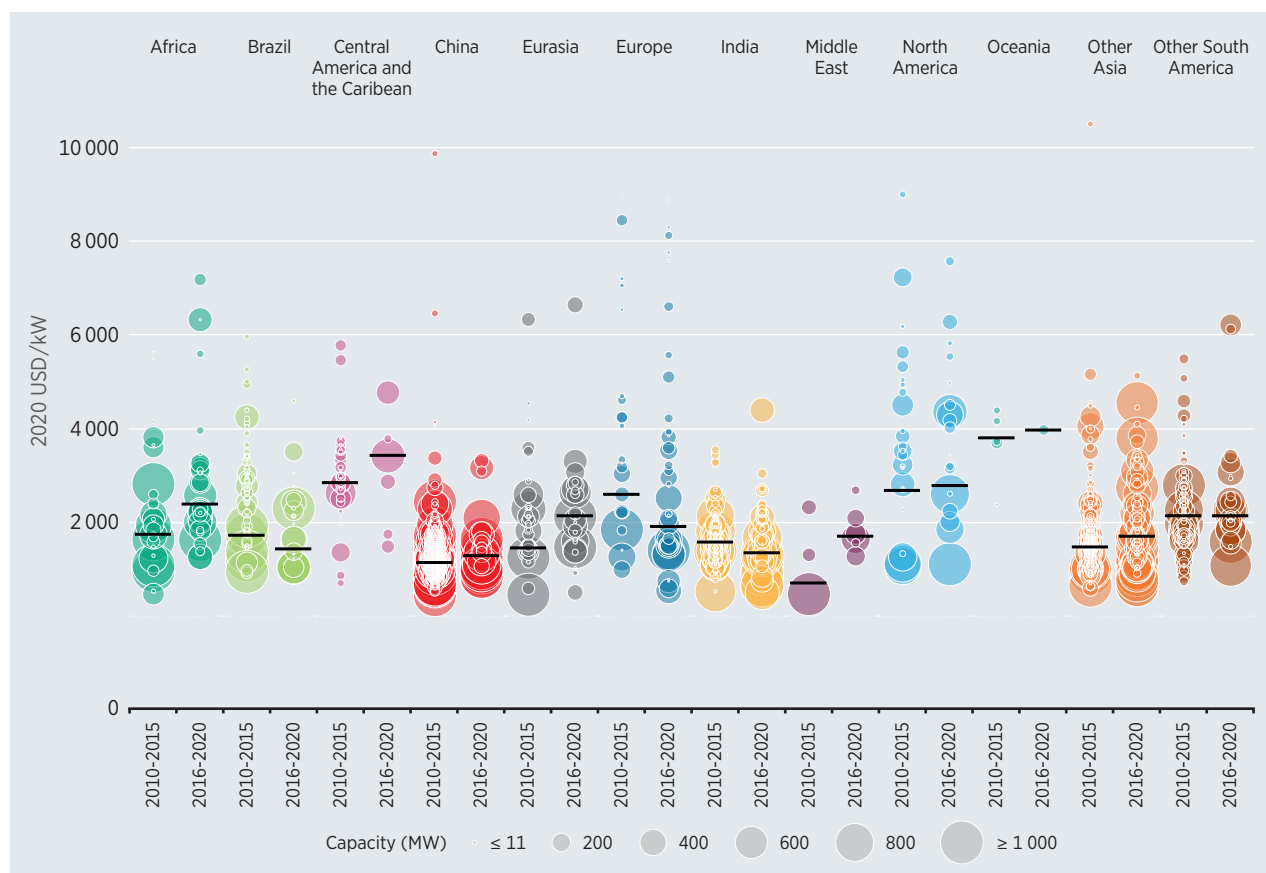
Figure 6.5 Total installed cost by project and capacity weighted averages for large hydropower projects by country/region, 2010-2020
