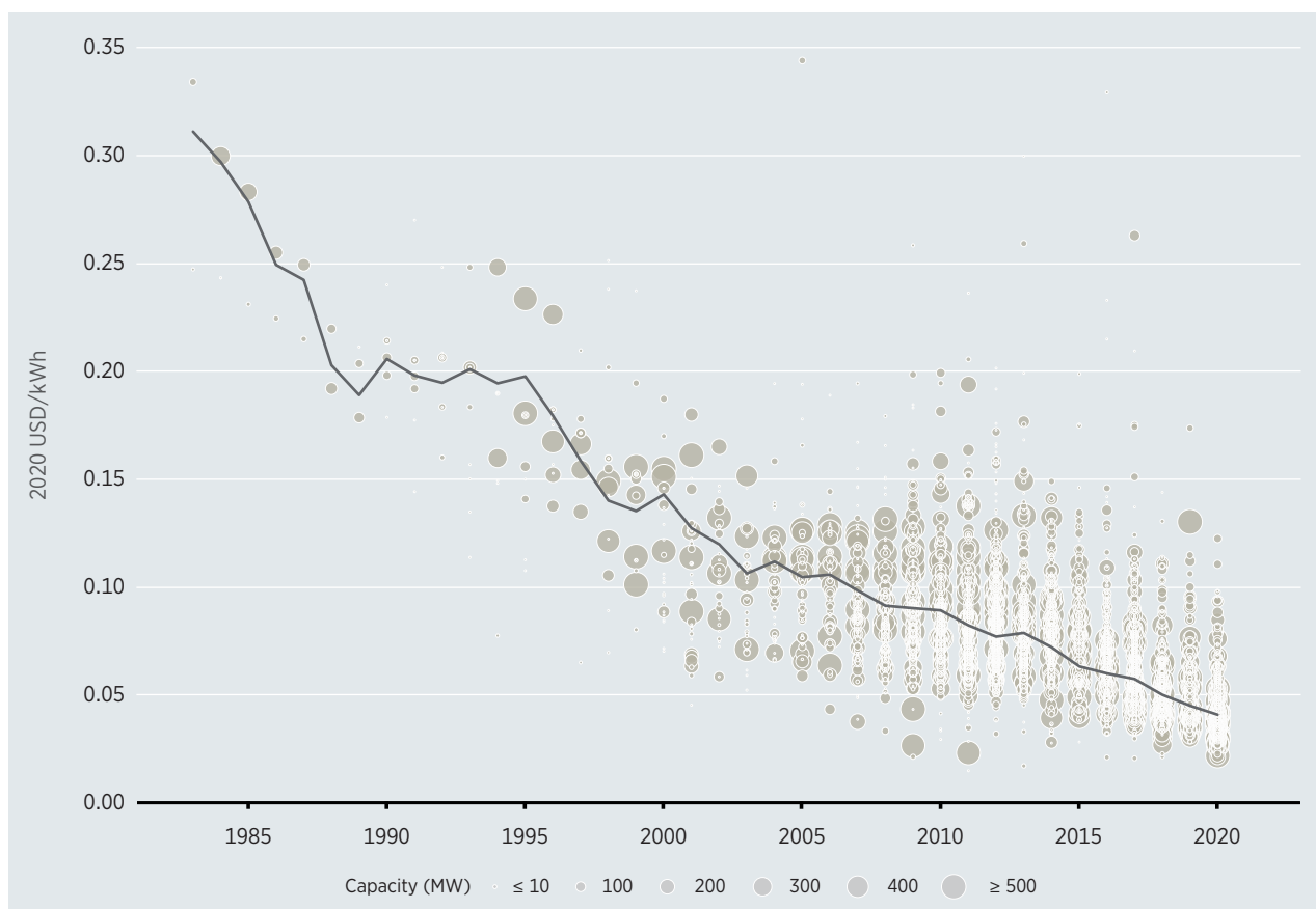
Figure 2.9 LCOE of onshore wind projects and global weighted average, 1983–2020
