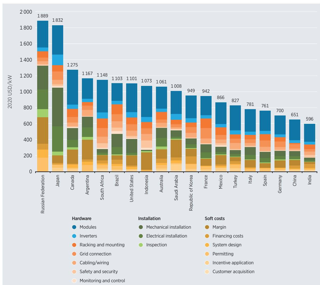
Figure 3.5 Detailed breakdown of utility-scale solar PV total installed costs by country, 2020
