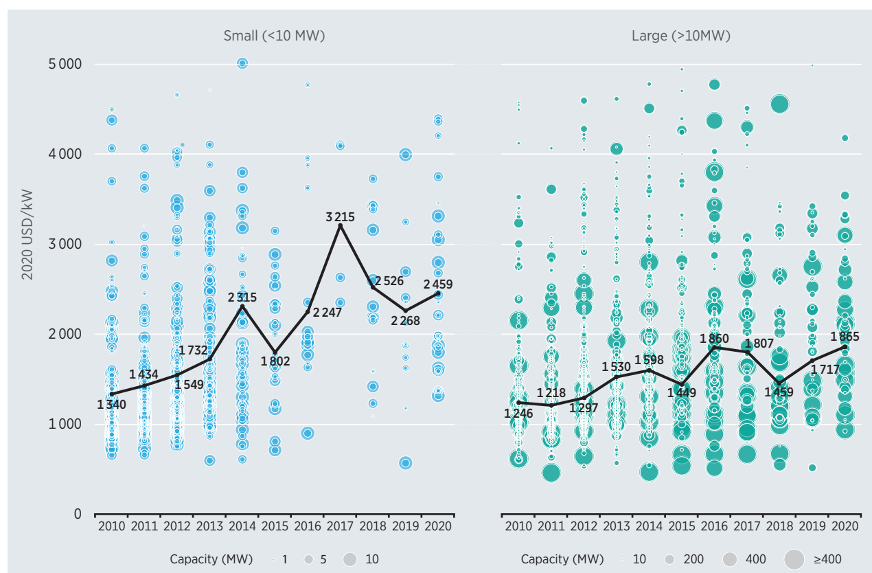
Figure 6.3 Total installed costs for small and large hydropower projects and the global weighted-average, 2010-2020
