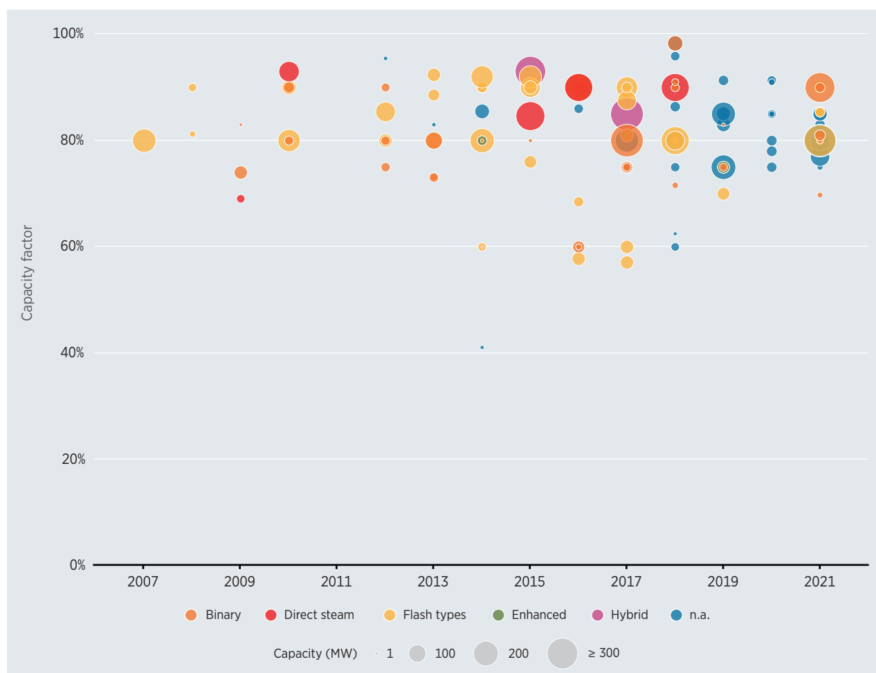
Figure 7.3 Capacity factors of geothermal power plants by technology and project size, 2007-2021
