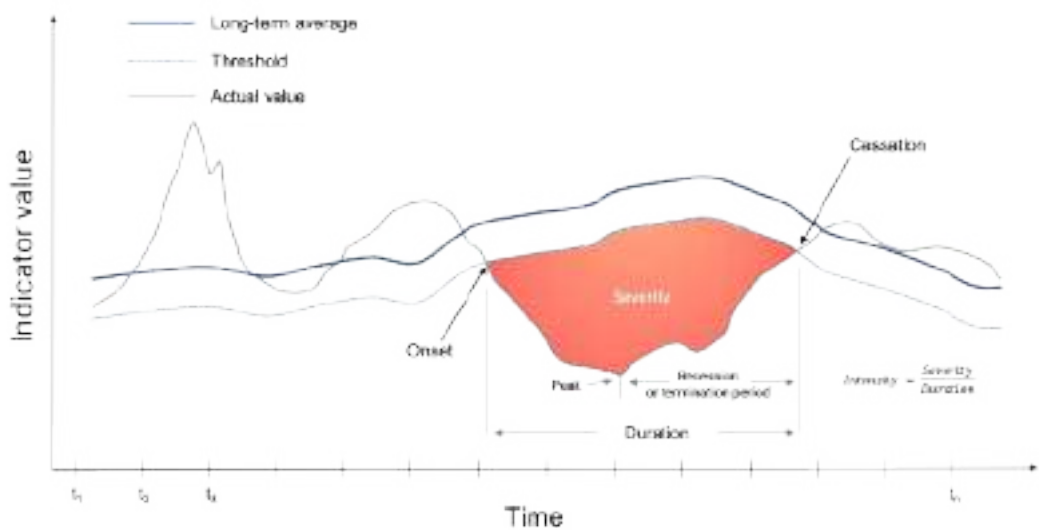
Figure 1.2. Schematic representation of selected key drought parameters
