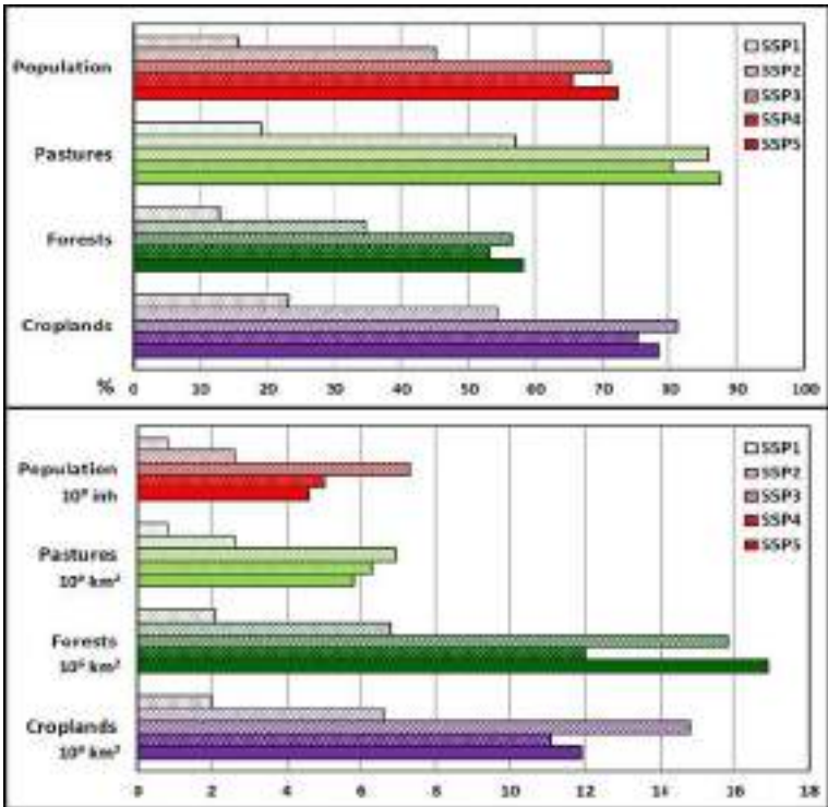
Figure 1.12. Percentage of areas (above) and total population and extent of land-use classes (below) subject to an increase in meteorological drought frequency and severity from 1981 to 2100 to the highest warming level allowed by five SSPs (1.5°C with SSP1, 2°C with SSP2, 3°C with SSP4, and 4°C with SSP3 and SSP5)
