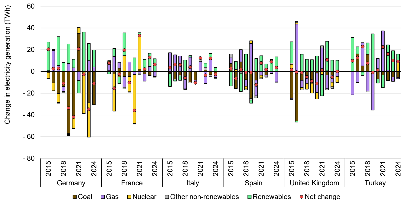
Change in electricity generation, 2015-2024
