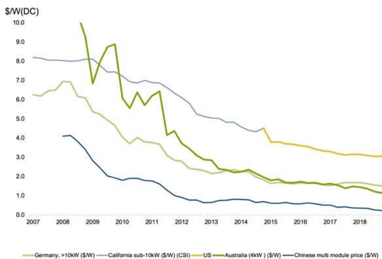
FIGURE 33. SMALL PV SYSTEM COST IN GERMANY, THE U.S. AND AUSTRALIA, AND TREND IN CHINESE MODULE PRICES, $ PER W
