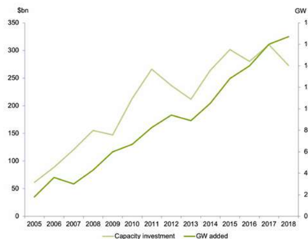
FIGURE 14. RENEWABLE ENERGY CAPACITY INVESTMENT IN $BN VS GW CAPACITY ADDED, 2005-2018
