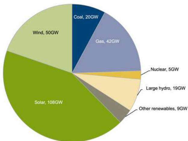
FIGURE 16. NET POWER GENERATING CAPACITY ADDED IN 2018 BY MAIN TECHNOLOGY, GW
