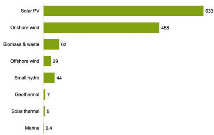
FIGURE 4. CAPACITY ADDED IN RENEWABLE POWER TECHNOLOGIES OVER THE DECADE, 2010-2019, GW
