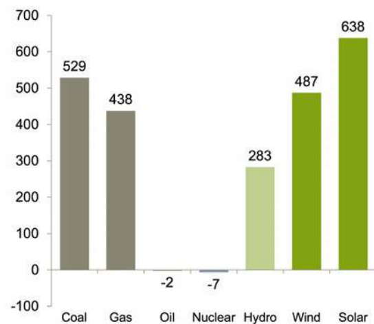
FIGURE 6. NET CAPACITY ADDED IN MAIN GENERATION TECHNOLOGIES OVER THE DECADE, 2019 VS 2009, GW
