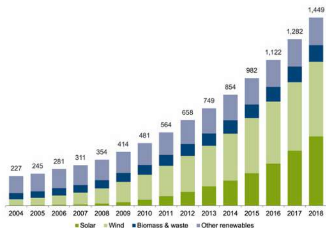
FIGURE 13. GLOBAL CAPACITY IN RENEWABLE POWER, 2004-2018, GW
