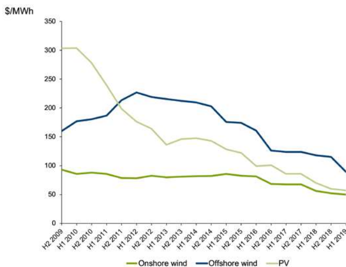
FIGURE 3. LEVELIZED COST OF ELECTRICITY, BY MAIN RENEWABLE ENERGY TECHNOLOGY, 2009 TO 2019, $/MWH
