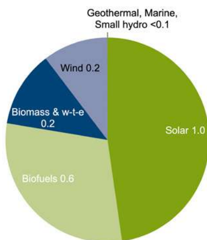
FIGURE 22. VC/PE NEW INVESTMENT IN RENEWABLE ENERGY BY SECTOR, 2018, $BN
