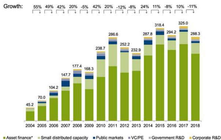
FIGURE 19. GLOBAL NEW INVESTMENT IN RENEWABLE ENERGY BY ASSET CLASS, 2004-2018, $BN
