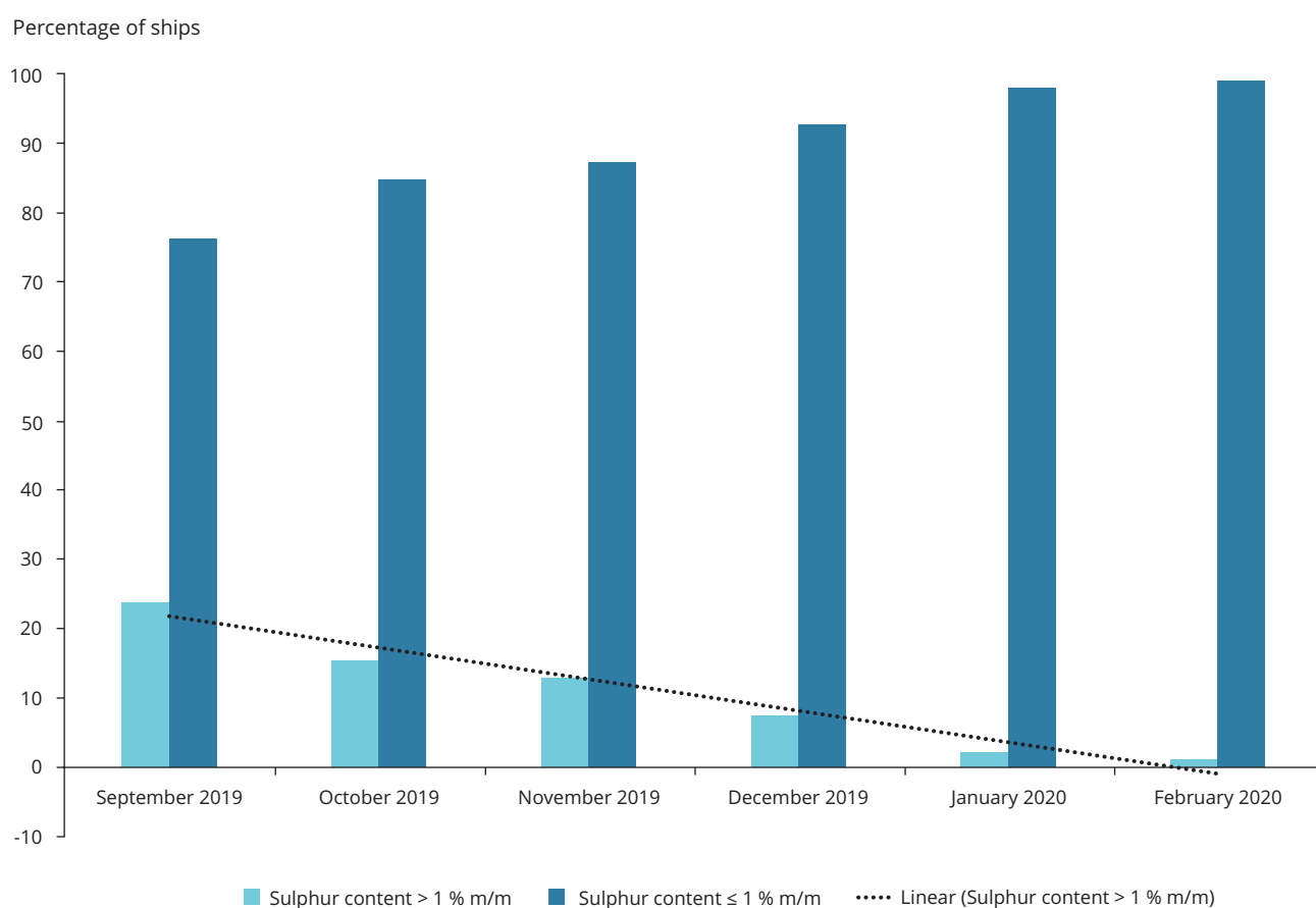
Figure 4.8 Monthly percentage of ships using residual fuels vs distillates
