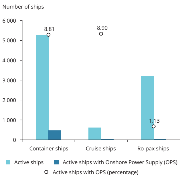
Figure 5.8 Percentage of active ships worldwide equipped with OPS
