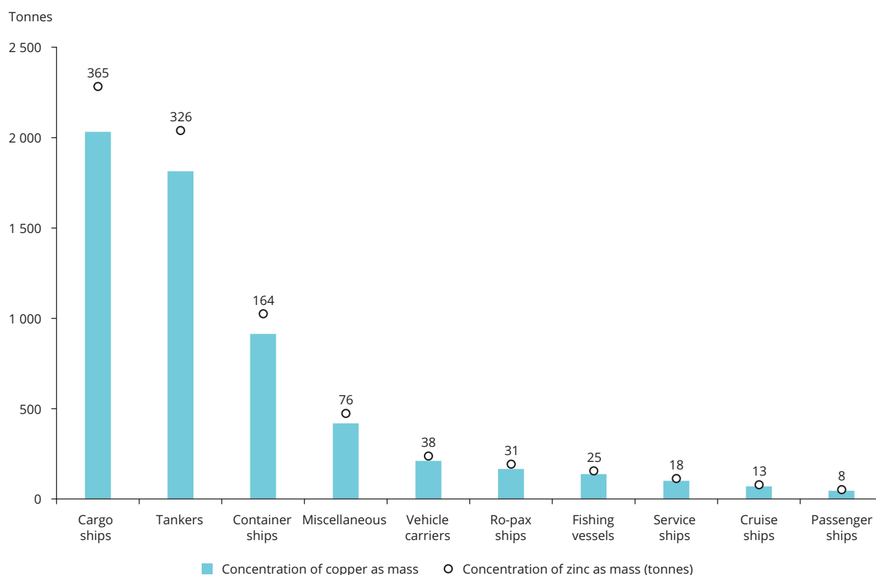
Figure 4.21 Estimated releases of the main copper and zinc compounds from anti-fouling paints, 2019
