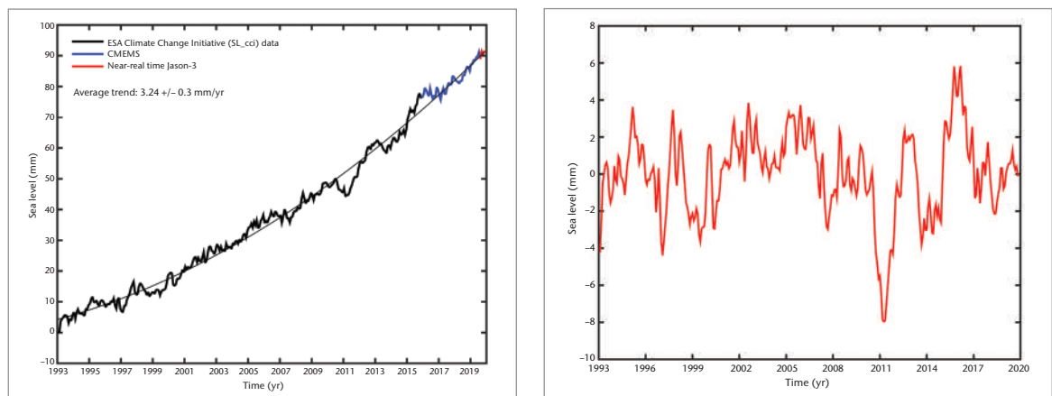
Figure 8. Left: Global mean sea-level evolution for January 1993–December 2019, from high-precision altimetry. The thin black curve is a quadratic function that best fits the data. The data from the Copernicus Marine Environment Monitoring Service (CMEMS) begin in January 2016 and those from the European Organization for the Exploitation of Meteorological Satellites (EUMETSAT) Jason-3 in October 2019. Right: Detrended global mean sea level over the same period (the difference between the smooth quadratic function and the measured values in the left panel).
