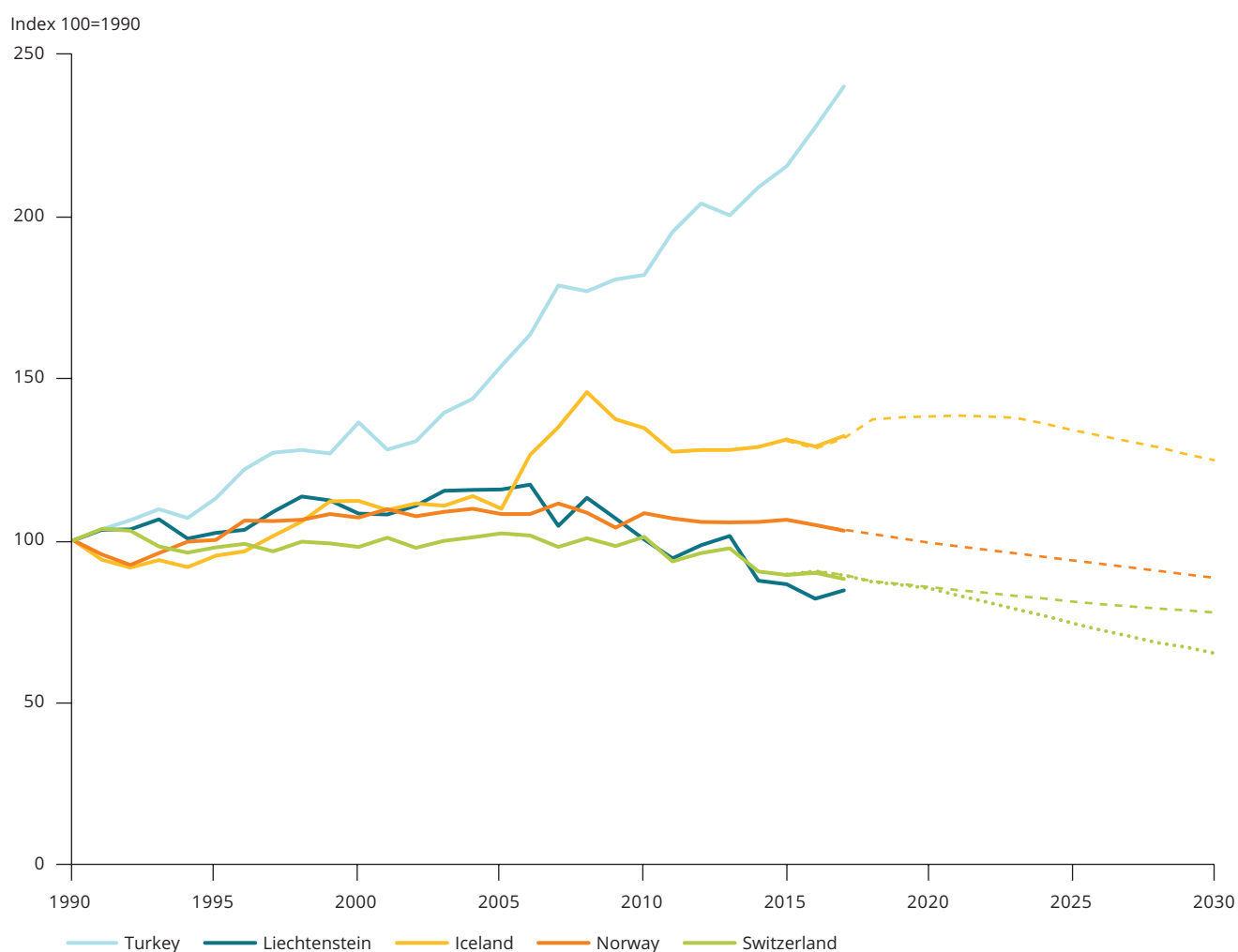
Figure 2.10 Total greenhouse gas emission trends and projections in Iceland, Liechtenstein, Norway, Switzerland and Turkey
