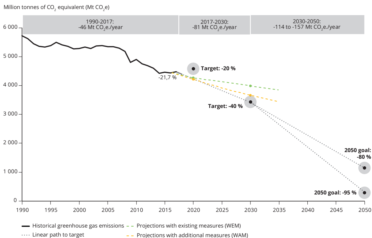
Figure ES.4 Greenhouse gas emission trends, projections and targets in the EU
