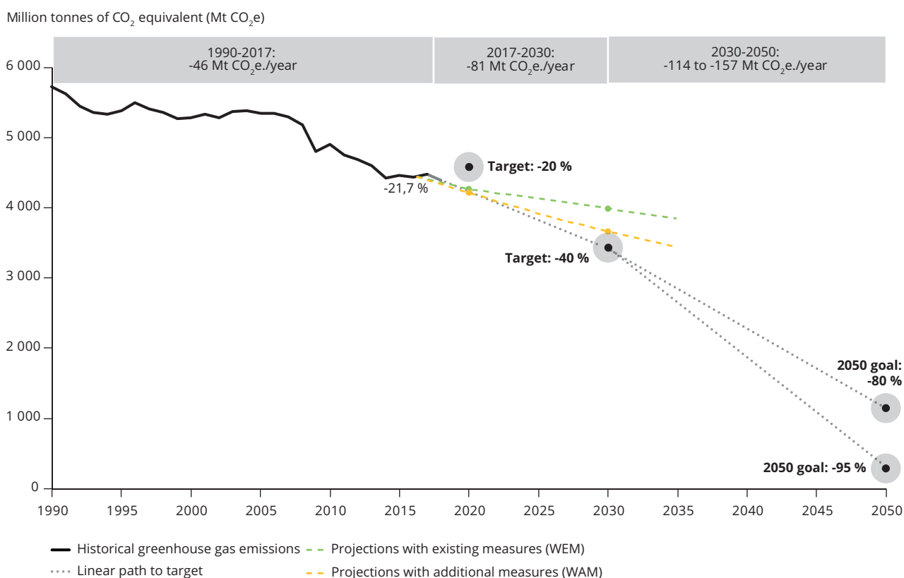
Figure 2.1 Greenhouse gas emission trends, projections and targets in the EU, 1990-2050
