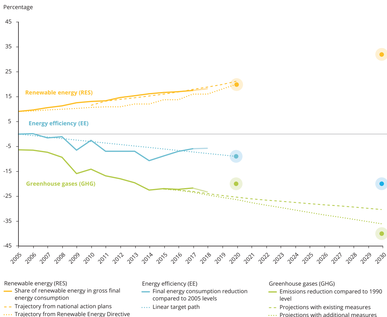
Figure ES.2 EU progress towards 2020 and 2030 targets on climate and energy
