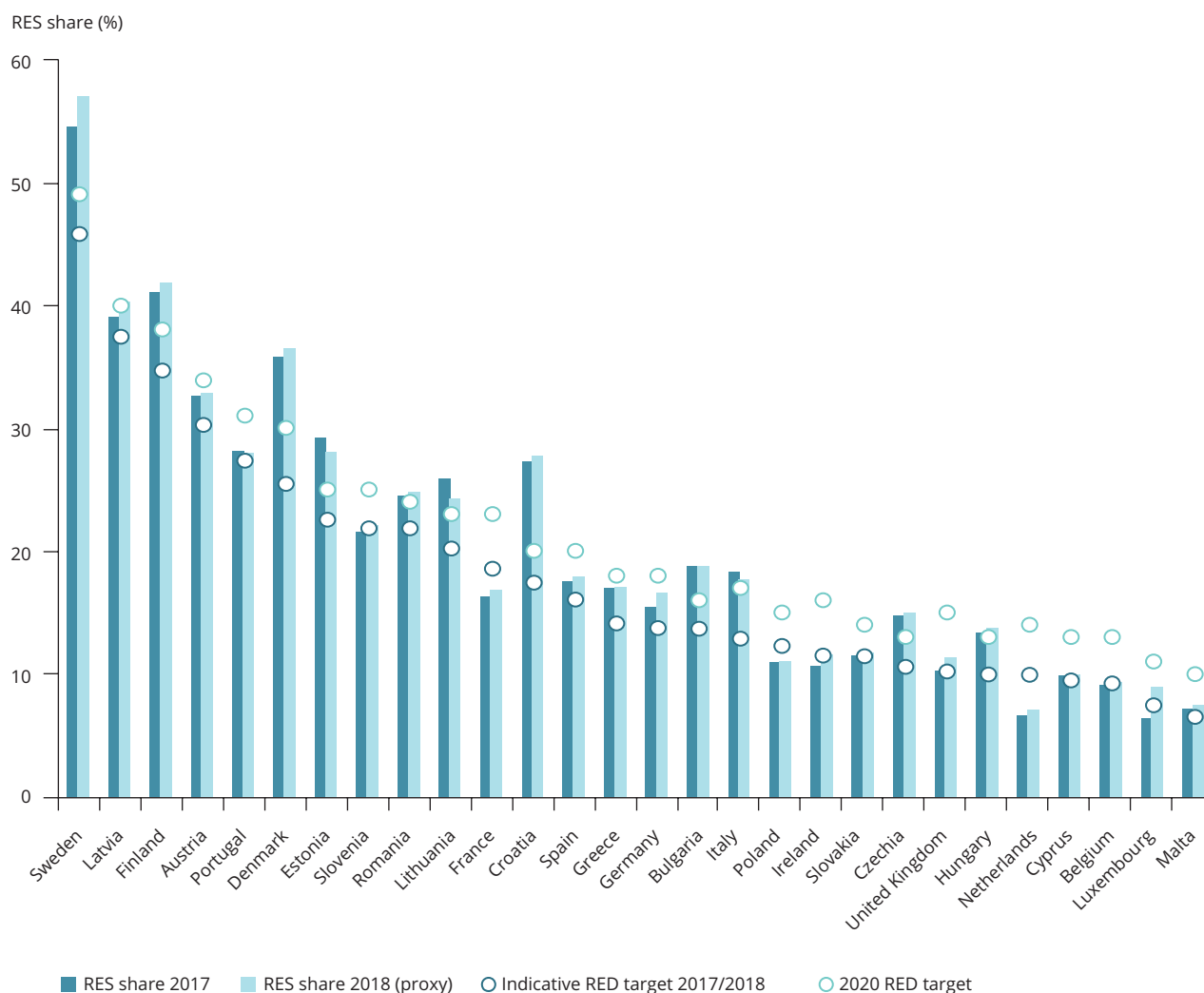
Figure 3.6 National shares of energy from renewable sources in relation to indicative trajectories set out in the Renewable Energy Directive
