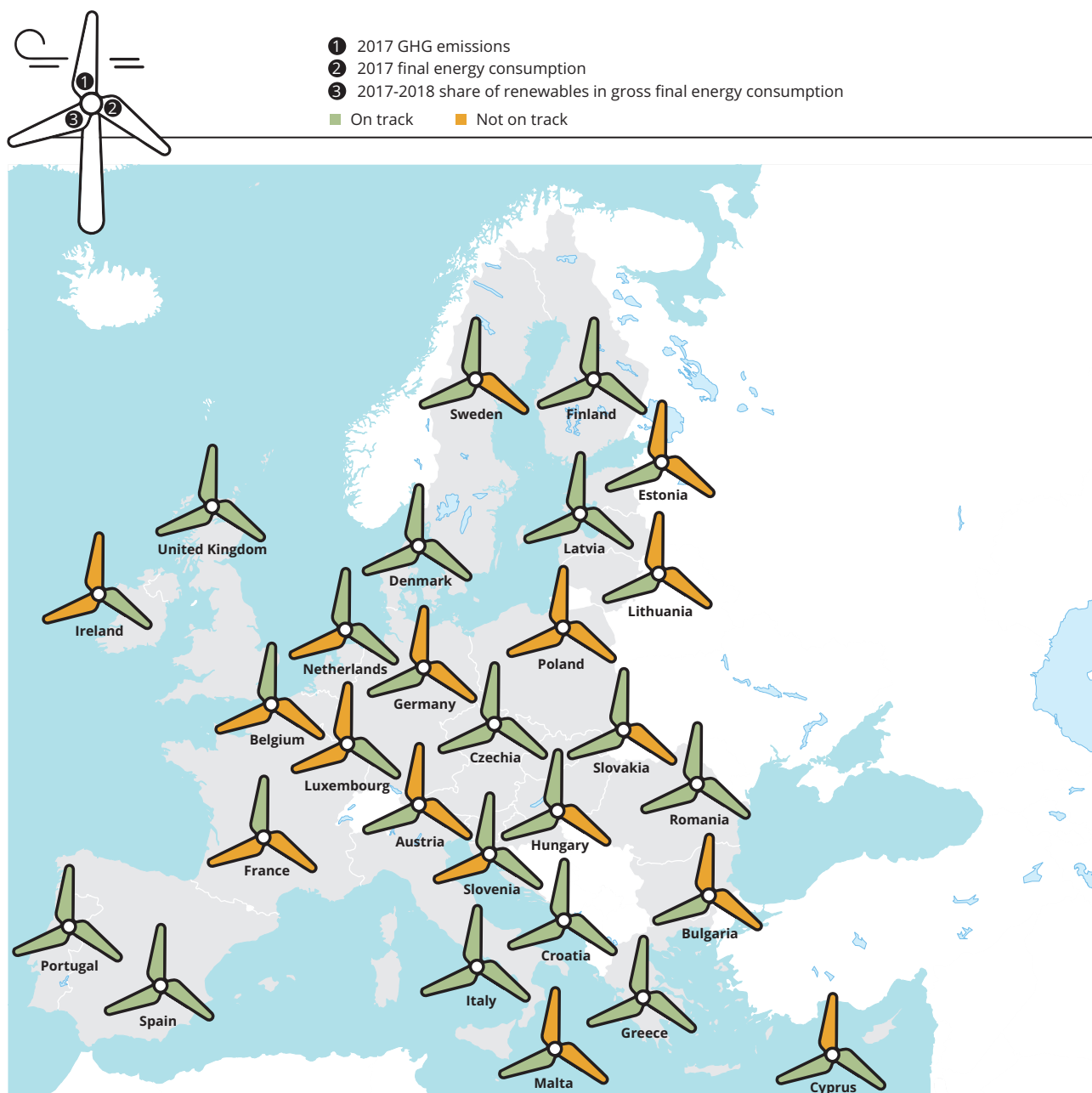
Figure ES.1 Current progress of Member States towards 2020 climate and energy targets
