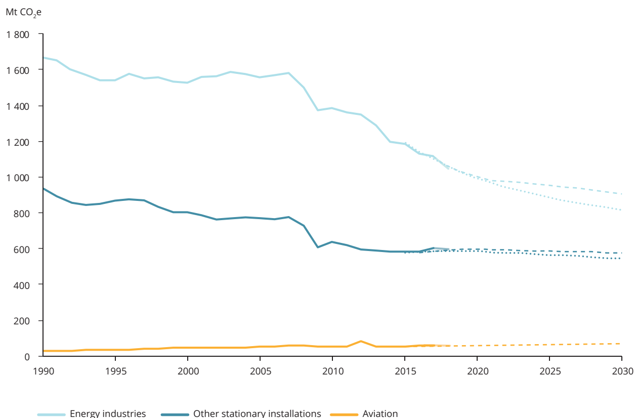
Figure 2.4 Greenhouse gas emission trends and projections under the scope of the EU ETS in the EU, 1990-2030
