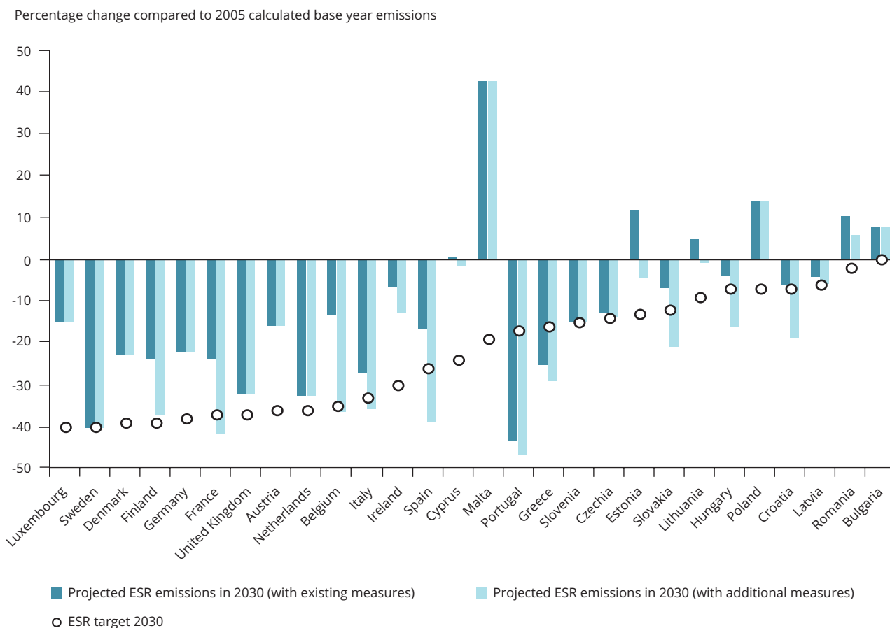
Figure 2.8 Projected progress of Member States towards their 2030 Effort Sharing targets
