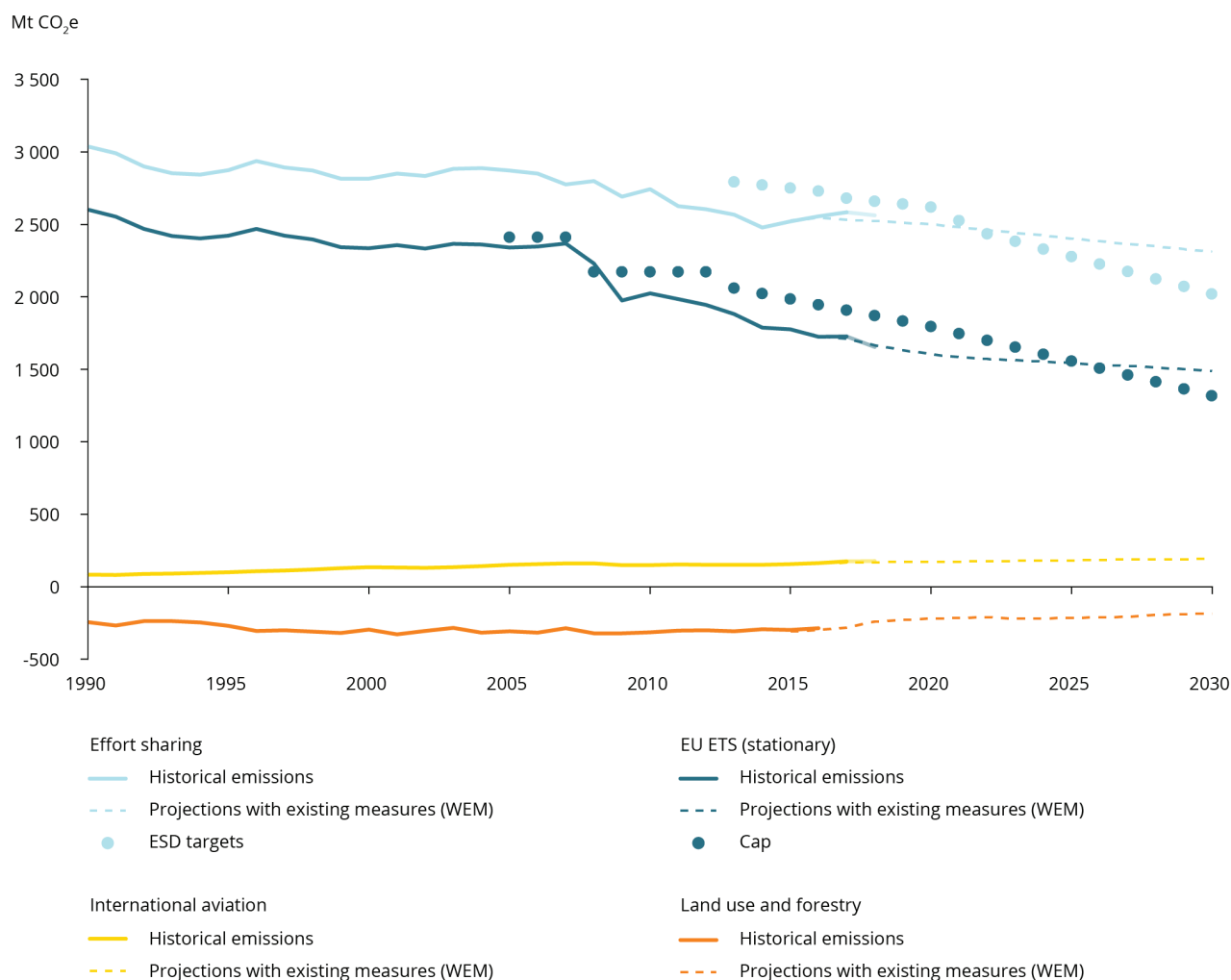
Figure 2.3 Effort Sharing, ETS, LULUCF and aviation emission trends and projections in the EU, 1990-2030
