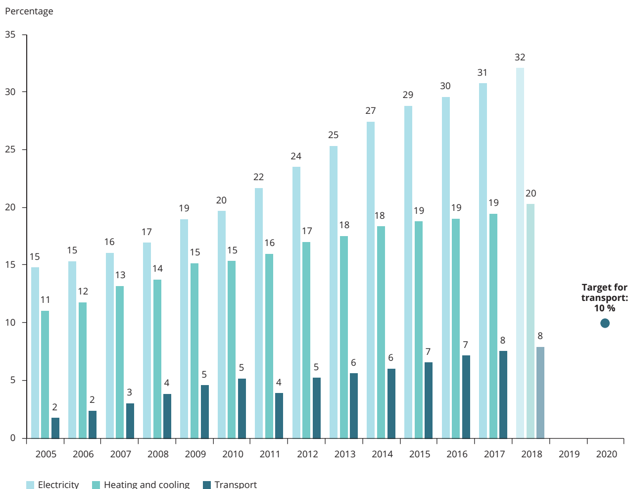
Figure 3.4 Shares of energy use from renewable sources by sector in the EU, 2005-2017 and proxy 2018
