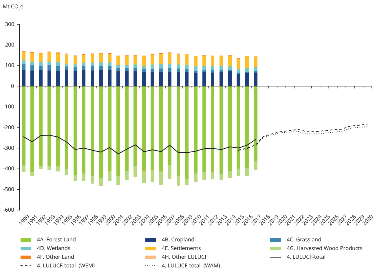
Figure 2.6 Reported EU LULUCF emissions and removals by land-use categories
