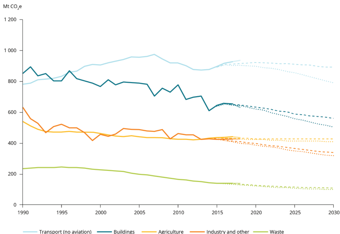
Figure 2.5 Greenhouse gas emission trends and projections under the scope of the Effort Sharing legislation
