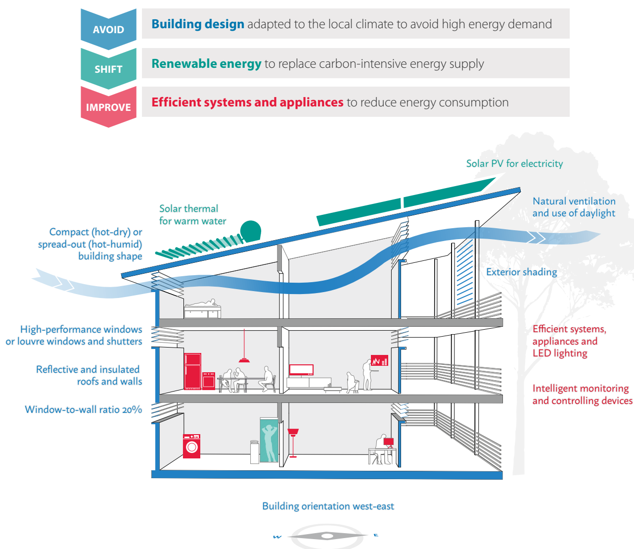
Figure 2 Energy efficiency measures in a building
