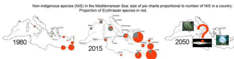
Figure 8 Non-indigenous species (NIS) in the Mediterranean Sea; size of pie charts proportional to number of NIS in a country; proportion of Lessepsian species in red 91 .
