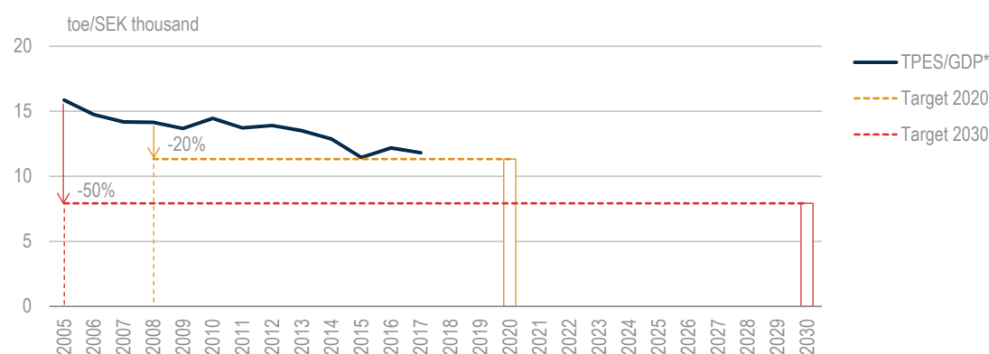
Figure 4.4 Energy intensity (TPES/GDP) 2005-17 and targets for 2020 and 2030
