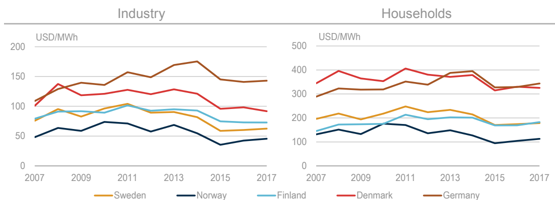
Figure 7.11 Electricity price trends in selected IEA member countries, 2007-17
